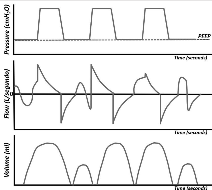
Figure 23. Pressure-time, flow-time, and volume-time curves.
