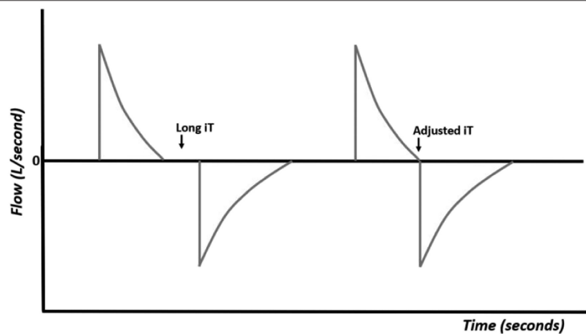
Figure 8. Flow-time curves with long iT and adjusted iT.
